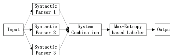
Figure 1: The pipeline of our system, where we combine the results of three dependency parsers and use max-entropy classifier to predict the semantic relations.
